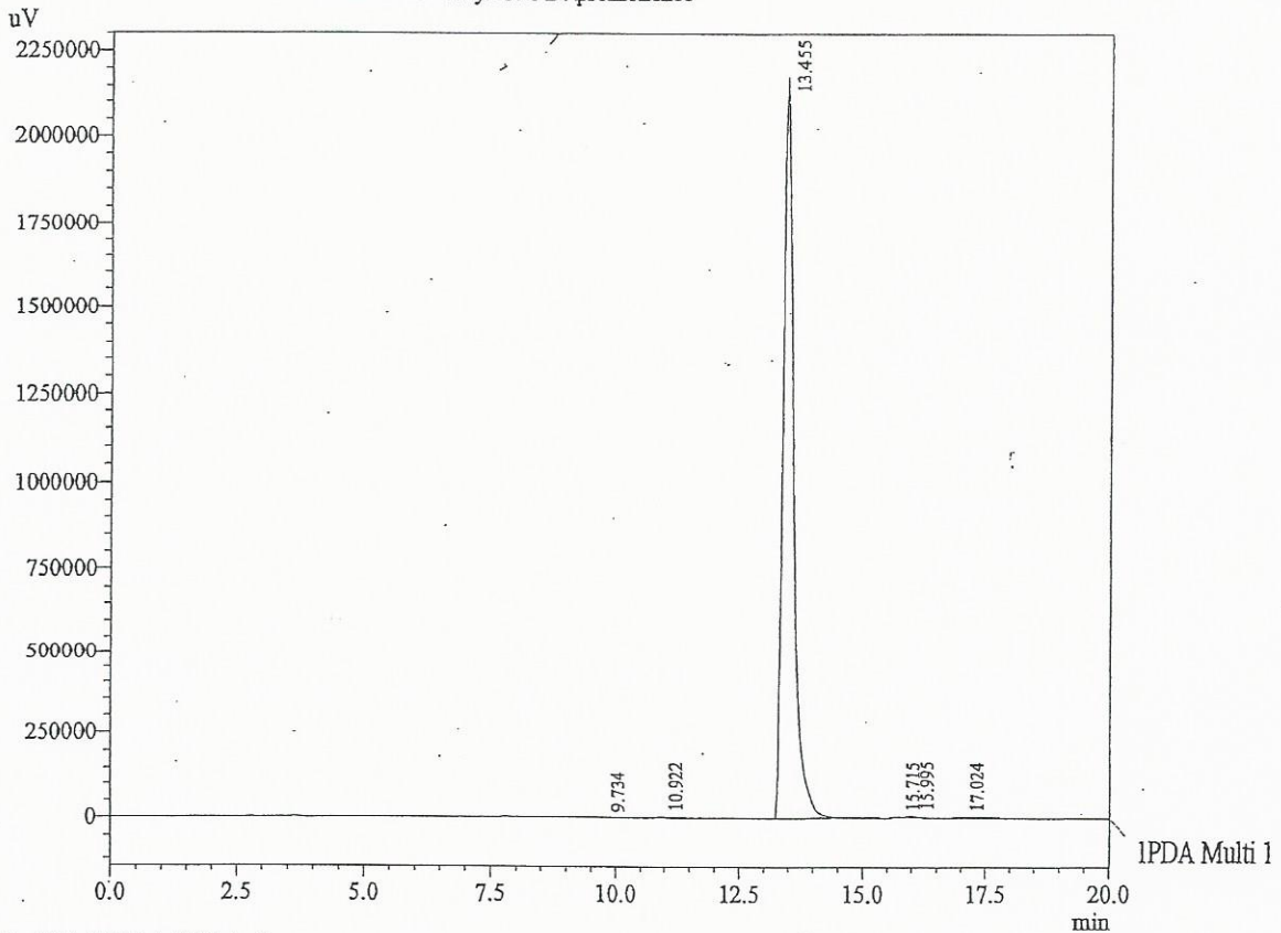
Chromatogram Vanilic acid ethylester D:\promonence
